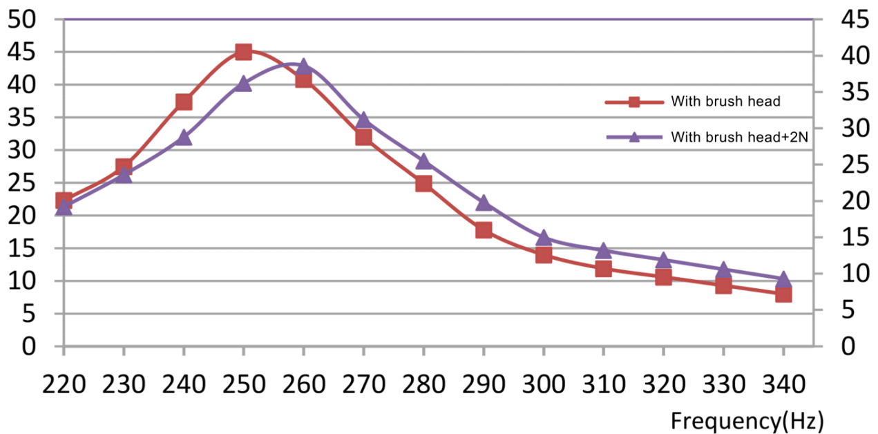
Angel(°) Frequency-angle curve
