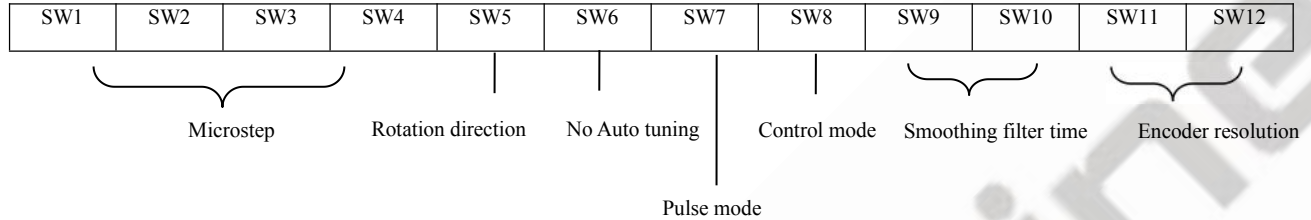
Figure 4: DIP switches
