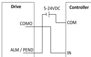
Figure 7 Sinking output
