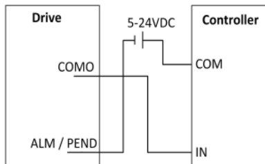
Figure 7 Sinking output
