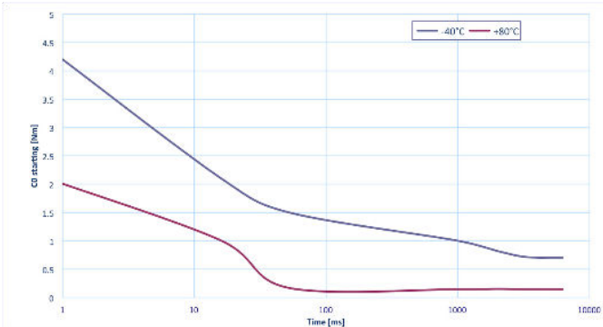
TETRA COMPACT-X 80 4 NO LOAD STARTING
