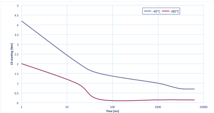
TETRA COMPACT-X 80 4 NO LOAD STARTING
