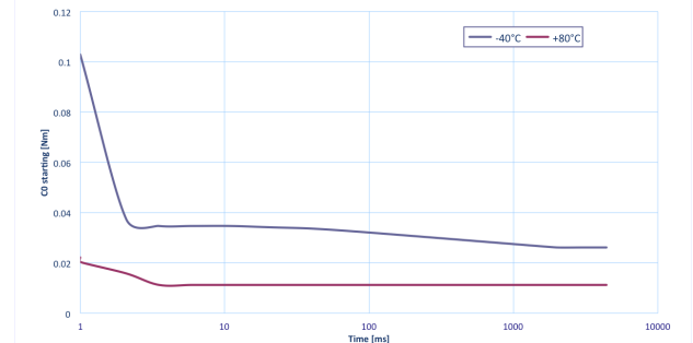
TETRA COMPACT-X 40 0,32 21 NO LOAD STARTING
