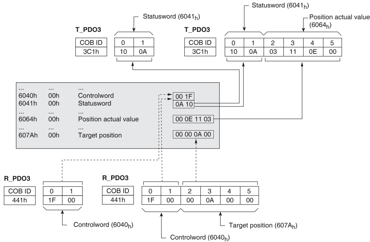
Figure 1.21 - PDO Mapping
