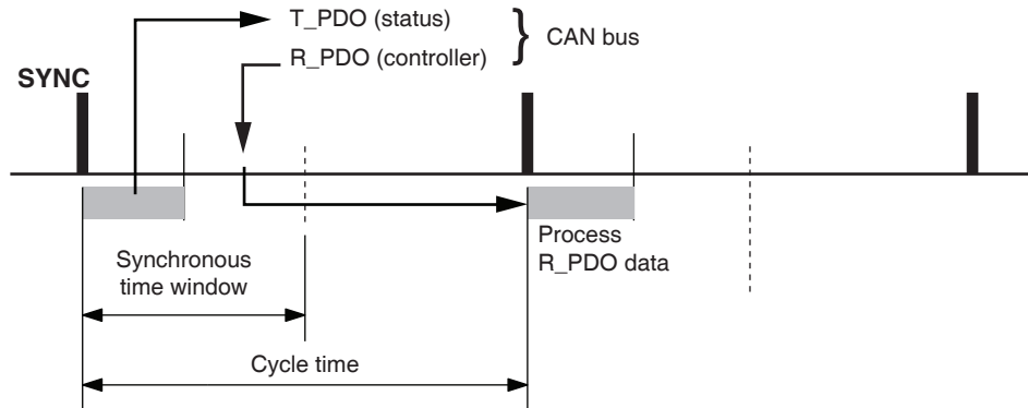
Figure 1.24 - Synchronization Times
