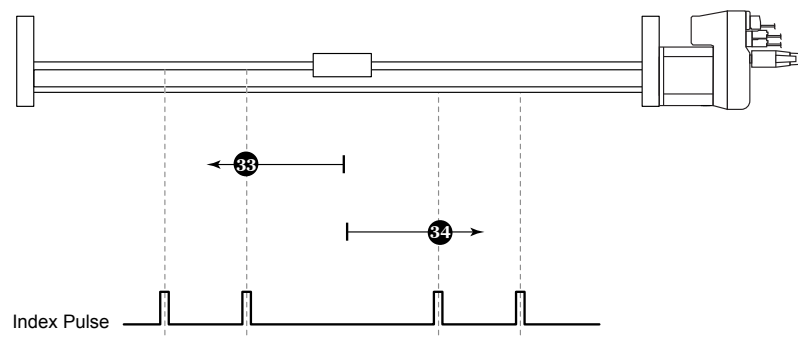
Figure 3.16 - Homing on an Index Pulse
