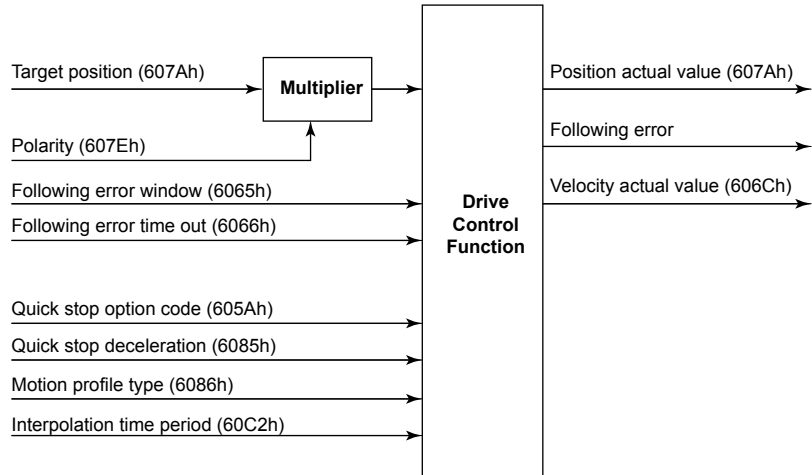
Figure 3.18 - Cyclic Synchronous Position Control Function
