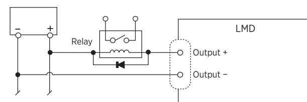
3. Inductive load
