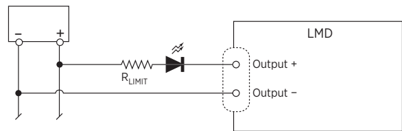
2. LED indicator Sinking
