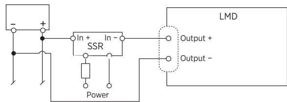
1. Solid state relay Sinking
