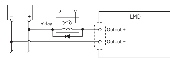
3. Inductive load Sinking
