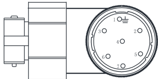
Motor side
