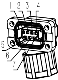
Motor side
