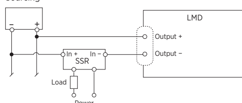
Sourcing
