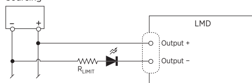
Sourcing
