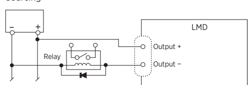
Sourcing
