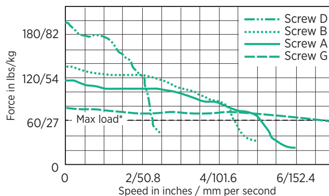
60 VDC
