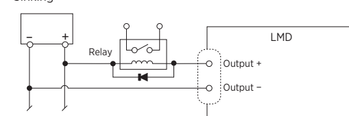
3. Inductive load Sinking
