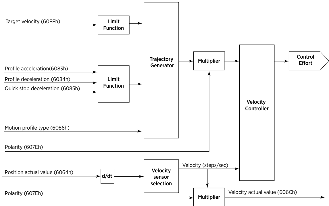
Figure 3.6 - Profile Velocity Control Function
