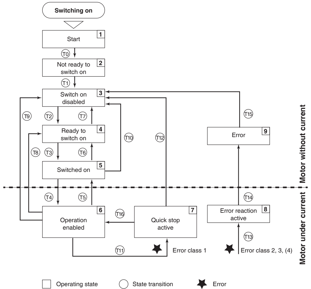
Figure 3.1 - State Diagram
