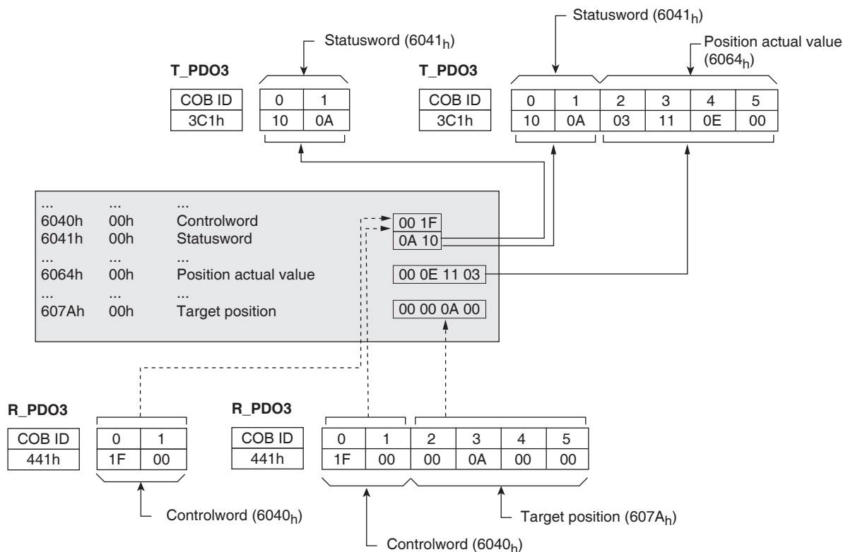
Figure 1.21 - PDO Mapping
