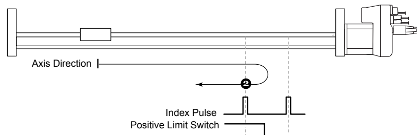
Figure 3.10 - Homing on the Positive Limit Switch and Index Pulse
