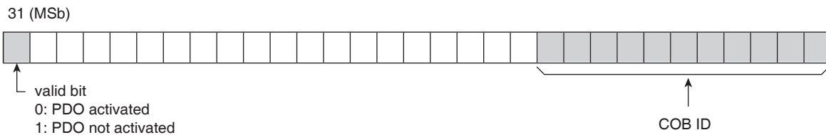
Figure 1.18 - Activating PDOs via Subindex 01 h , Bit 31
