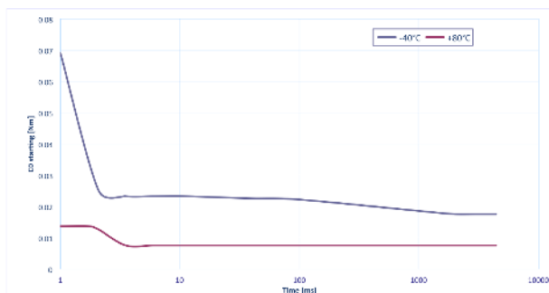
TETRA COMPACT-X 40 0,16 NO LOAD STARTING
