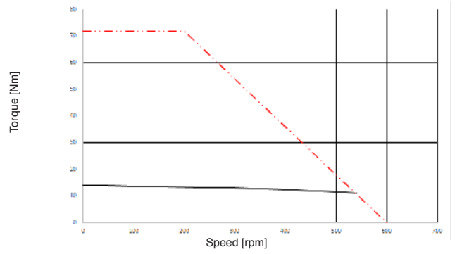
SKA DDR 148.120.19 400 Vac
