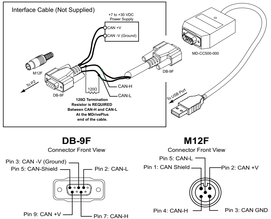
Figure 6.2 MD-CC500-000 USB to CANopen commissioning cable
