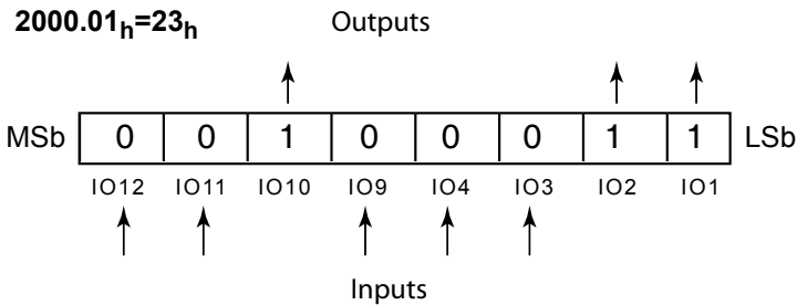
Figure 8.11: I/O structure
