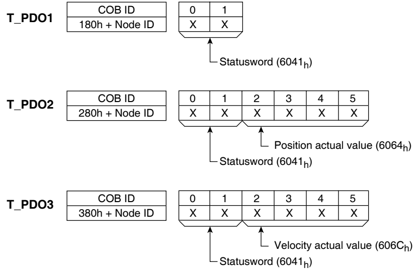
Figure 3.17 Transmit PDOs
