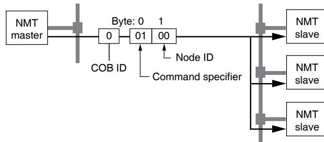
Figure 3.27 NMT message
