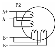
Figure 9: 8-lead motor parallel connections
