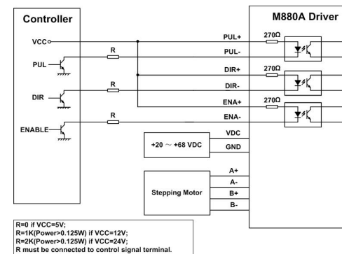
Figure 10: Typical connection
