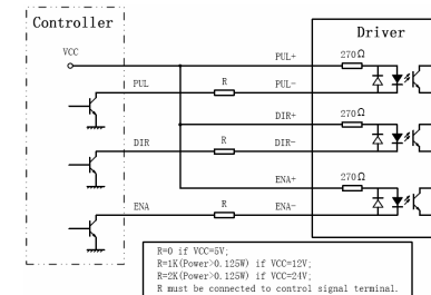
Figure 3: Connections to open-collector signal (common-anode)
