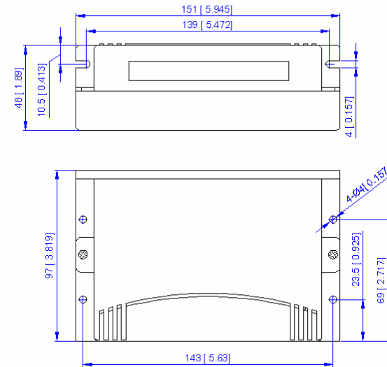
Figure 1: Mechanical specifications
