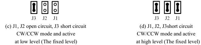
Figure 2: J1 and J3 jumpers
