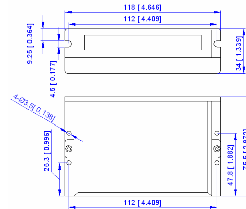
Figure 1: Mechanical specifications
