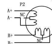
Figure 7: 6-lead motor full coil (higher torque) connections
