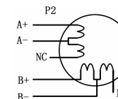
Figure 6: 6-lead motor half coil (higher speed) connections
