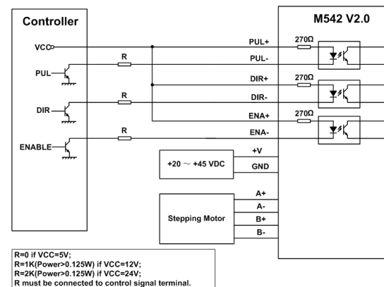
Figure 10: Typical connection
