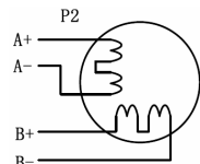
Figure 5: 4-lead Motor Connections
