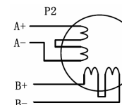
Figure 8: 8-lead motor series connections
