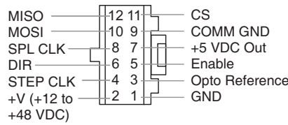
Figure A.7 Connector kit CK-08
