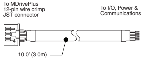
Figure A.6 Prototype development cable PD12B-3400-FL3
